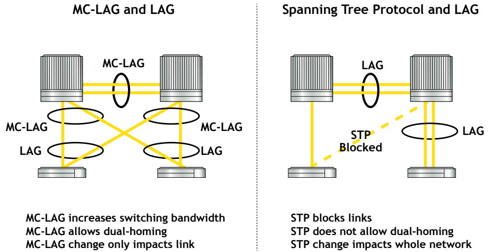
Figure 4. MC-LAG versus spanning tree protocol
